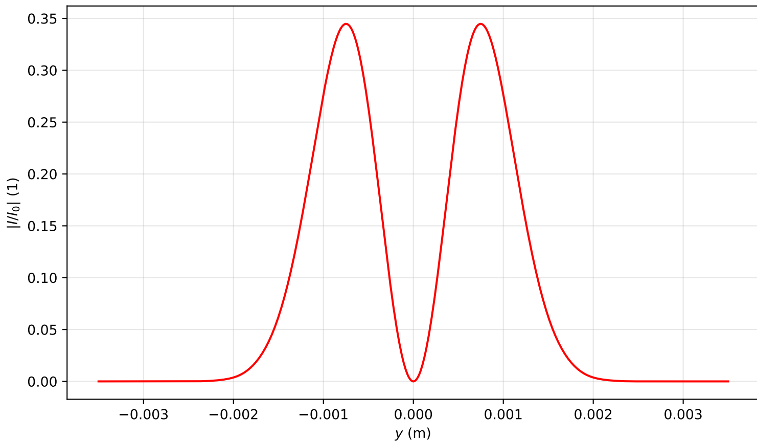
Intensity profile I(x=0, y, z=2.309)/I_0 , P_{in}=0.5P_{cr} , artificial time
